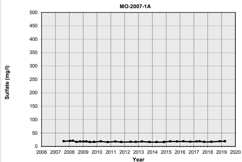
FIGURE C.5 SULFATE CONCENTRATION OVER TIME FOR WELLS MO-2007-1A, MO-2007-1B, AND MO-2007-1C
